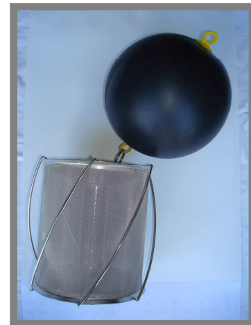
Fine filter housing with .047 mesh and 2" (51) connection (WISY SZ9931)
