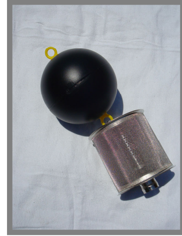
Fine filter housing with .047 mesh and 1 1/4" (32) connection (WISY SZ9936)
